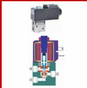
3 way High Orifice Solenoid Valve
